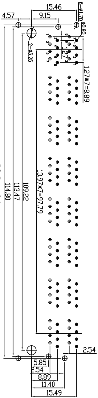
PC Board Layout
